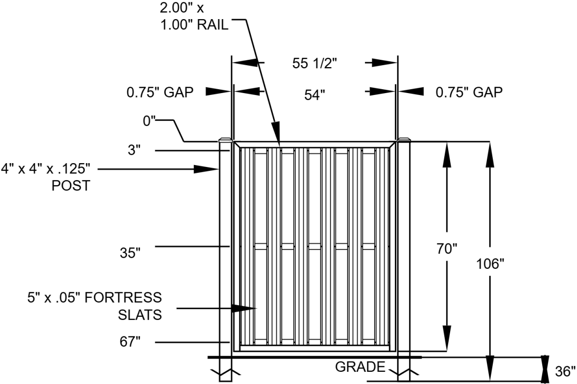
6ft H by 55.5inW - GATE -Commercial Aluminum Semi-privacy Fence - Shadowbox
