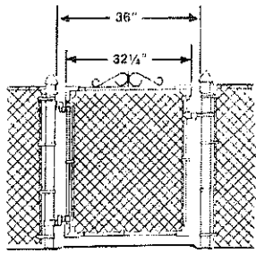
3' WALK GATE
